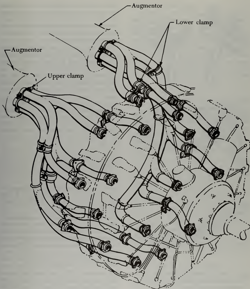
FIGURE 2-32. Exhaust manifold installation.
